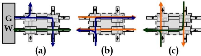
Figure 7. Gateway (a), injection (b), and ejection (c) switches. All possible message-paths are marked to demonstrate that no blocking interactions occur
