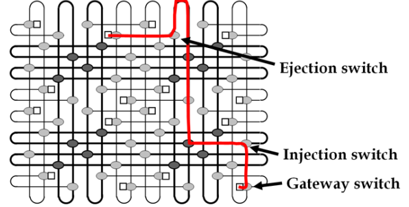
Figure 5. Example of a deadlock-avoiding path on the augmented folded torus network.
